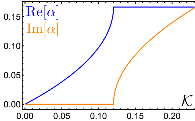
FIG. 12: Plot of \text{Re}[\alpha] and \text{Im}[\alpha] , for the solutions which have \text{Re}[\alpha] \leq 1/6 and \text{Im}[\alpha] > 0 , as a function of \mathcal{K} . For 1 > \mathcal{K} > \mathcal{K}^* , \text{Re}[\alpha] = 1/6 and \text{Im}[\alpha] \neq 0 .
