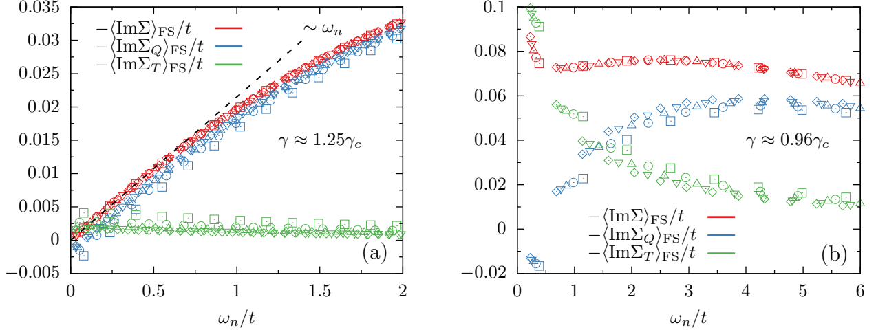
FIG. 3: (a) Imaginary part of the fermion self-energy averaged over the Fermi surface, as a function of Matsubara frequency, \omega_n , on the Fermi liquid side ( \gamma \simeq 1.25\gamma_c ) for \beta t = 40 - 100 . Red shows the full self-energy, -\langle \text{Im}\Sigma \rangle_{\text{FS}} , while blue and green show the quantum, -\langle \text{Im}\Sigma_Q \rangle_{\text{FS}} , and thermal, -\langle \text{Im}\Sigma_T \rangle_{\text{FS}} , contributions, respectively. Different symbols correspond to different temperatures. For the full \Sigma , the points for various temperatures fall essentially on the same curve, indicating \Sigma has converged to its T = 0 value. The components \Sigma_Q and \Sigma_T show a more significant temperature dependence. We find -\text{Im}\Sigma \sim \omega_n at small frequency, consistent with a Fermi liquid. In this regime, the contribution from \Sigma_T is small. (b) Same as (a) but on the ordered side ( \gamma \simeq 0.96\gamma_c ) for \beta t = 8 - 14 . In this regime -\text{Im}\Sigma is an increasing function of \omega_n at small frequency, where it is dominated by \Sigma_T .
