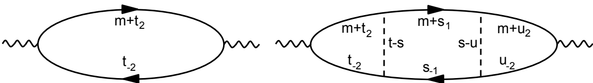
FIG. 19: Tree level (left) and leading correction (right) to the propagator for the operator \psi_2^{1\dagger}\psi_2^3 . The subscripts show the hot spot involved. 1 and -1 correspond to the a = 1 hot spots of the \ell = 1 and \ell = 3 pair of hot spots, respectively. Similarly, 2 and -2 correspond to the a = 2 hot spots of the \ell = 1 and \ell = 3 pair.
