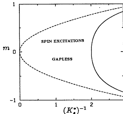
FIG. 1. Plot of the regions in which y_s is relevant or irrelevant for the Hamiltonian H_b as a function of m and K_s^* . The dashed line indicates the limit on the values of |m| above which H_b is not positive definite.
