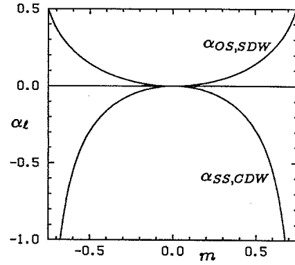
FIG. 2. Exponents \alpha_l as a function of the coupling m for the case K_\sigma and K_\rho=1 , K_s^*=0.5 , v_s^*=1 , v_\sigma=0.3 . Positive values of \alpha_l correspond to quasi-long-range order in the corresponding order parameter.
