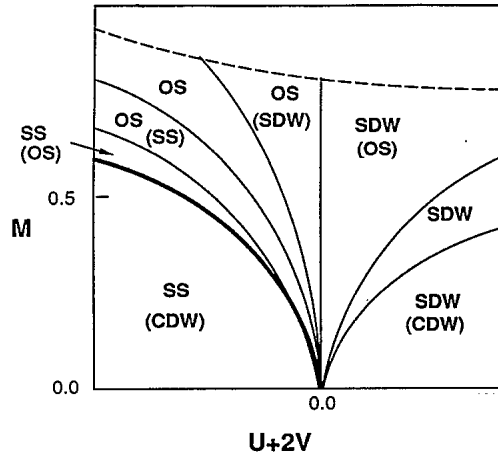
FIG. 3. Schematic phase diagram of H' as a function of M and U+2V . The Hamiltonian H corresponds to the vertical line U+2V=0 . If a given phase has two types of divergent fluctuations, the less divergent one is indicated in brackets. The dark line is a Kosterlitz-Thouless-type transition, while all other phase boundaries correspond to the order parameter exponents a_i continuously passing through zero. The dashed line is the limit of stability of H'_b .
